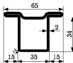
ZP 1604 M=3,00kg/m SERIES 34
