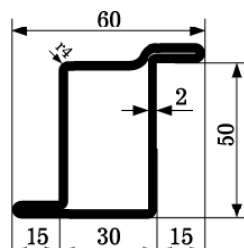
ZP 1221 M=3,24kg/m SERIES 50
