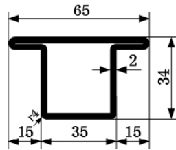
ZP 1004 M=2,83kg/m SERIES 34
