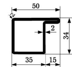
ZP 1304 M=2,40kg/m SERIES 34
