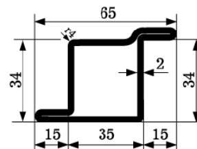
ZP 1204 M=2,90kg/m SERIES 34
