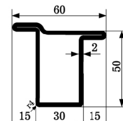
ZP 1121 M=3,24kg/m SERIES 50
