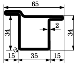
ZP 1104 M=2,90kg/m SERIES 34
