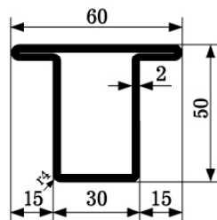
ZP 1021 M=3,13kg/m SERIES 50
