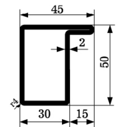
ZP 1321 M=2,75kg/m SERIES 50
