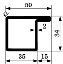
ZP 1304 M=2,40kg/m SERIES 34
