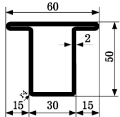
ZP 1021 M=3,13kg/m SERIES 50
