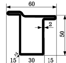
ZP 1121 M=3,24kg/m SERIES 50
