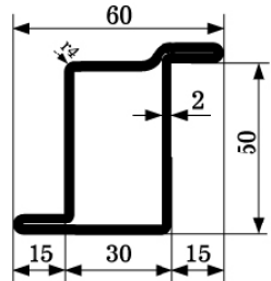
ZP 1221 M=3,24kg/m SERIES 50
