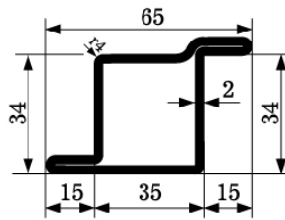
ZP 1204 M=2,90kg/m SERIES 34
